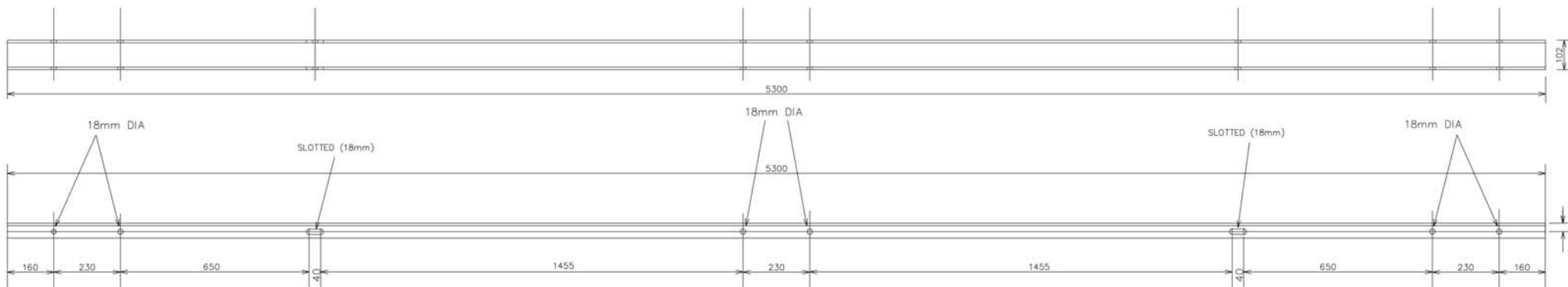
ITEM 12 102 x 51 x 5300mm LONG SURGE ARRESTOR SUPPORT CHANNEL
