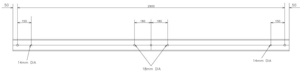
ITEM 13 127 x 64 x 3000mm LONG CABLE SUPPORT CHANNEL
