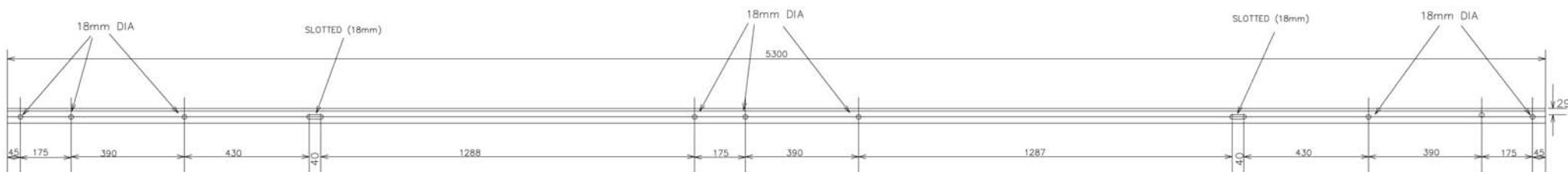
ITEM 11 102 x 51 x 5300mm LONG CABLE TERMINATION SUPPORT CHANNEL
